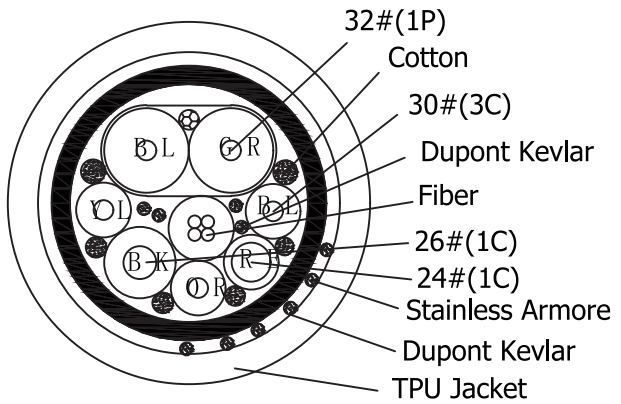
Armored HDMI Active Optical Cable (4 Fiber+7 Copper wire) Black TPU OD:5.8MM
