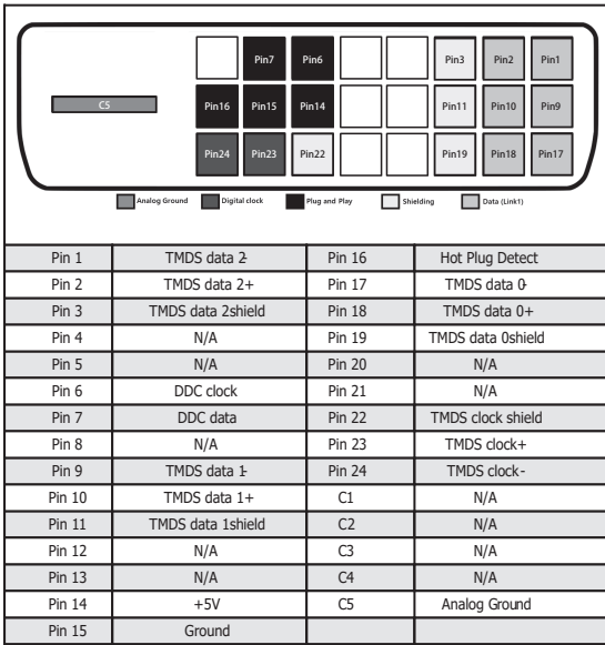
<Male DVI-D Single Link Pin Assignment>
